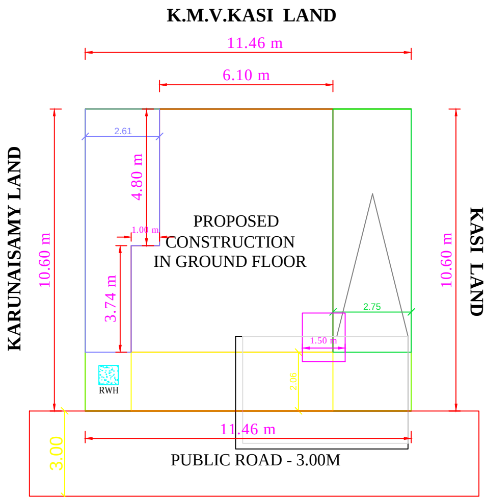
SITE PLAN
