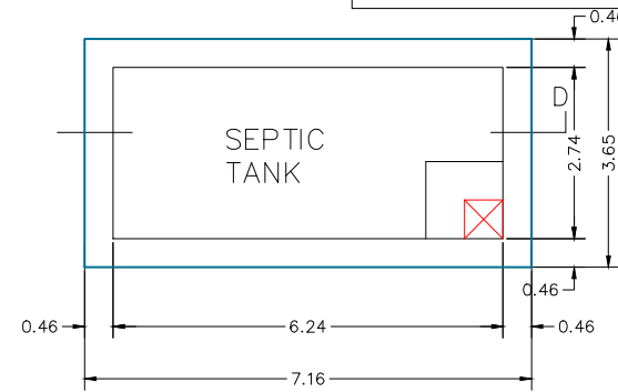
PLAN OF SEPTIC TANK SCALE 1"=2'0"
