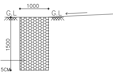
SECTION OF PEBBLE TRENCH SCALE : 1: = 100
