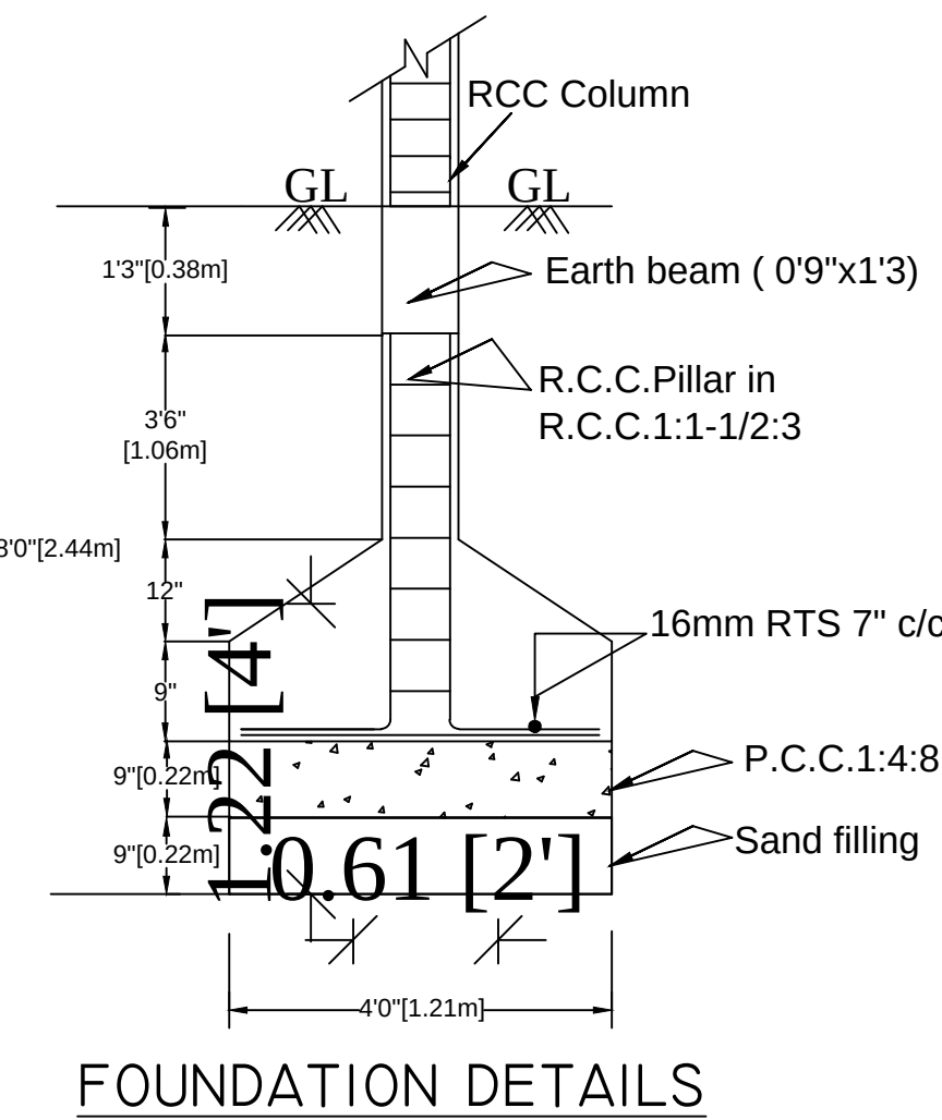
FOUNDATION DETAILS
