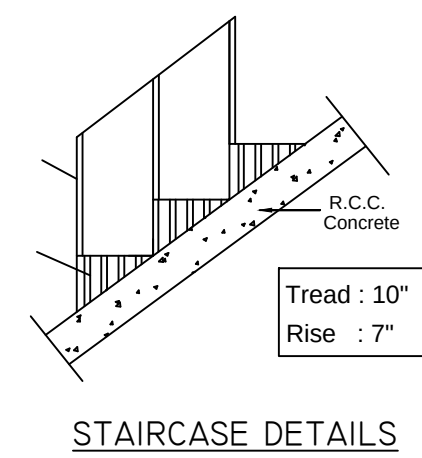
STAIRCASE DETAILS
