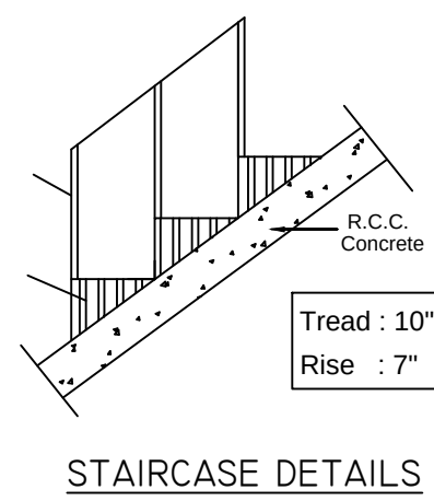
STAIRCASE DETAILS
