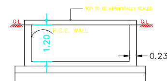
RWH SECTION (SAMPLE) RWH_CAPACITY_L = 2000LTRS
