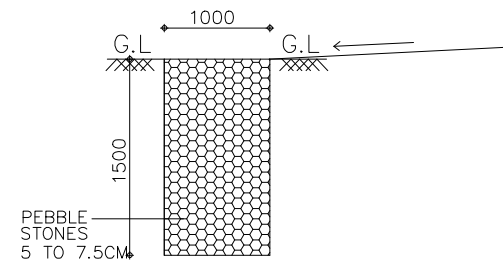
SECTION OF PEBBLE TRENCH SCALE : 1: = 100
