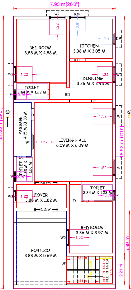
GROUND FLOOR PLAN [ WEST FACING ]
