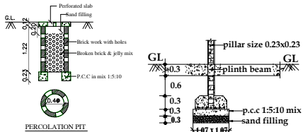
FOUNDATION DETAILS
