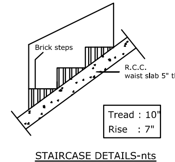
STAIRCASE DETAILS-nts
