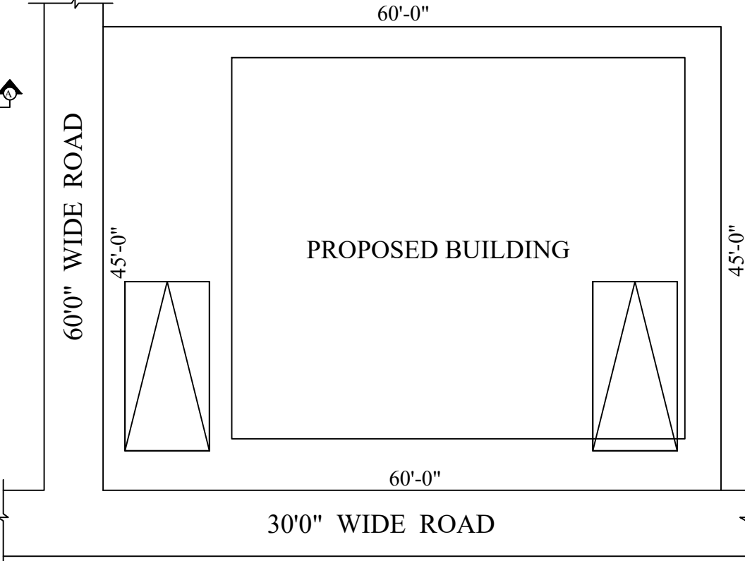
SITE PLAN
