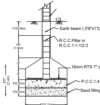
FOUNDATION DETAILS
