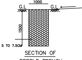
SECTION OF PEBBLE TRENCH
