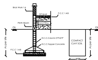
FOUNDATION DETAILS
