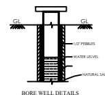
BORE WELL DETAILS
