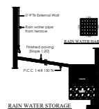
RAIN WATER STORAGE
