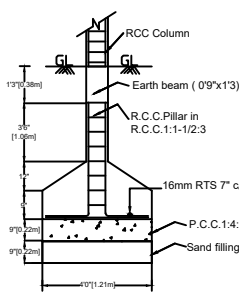
FOUNDATION DETAILS
