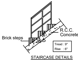
STAIRCASE DETAILS
