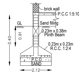
FOUNDATION DETAILS
