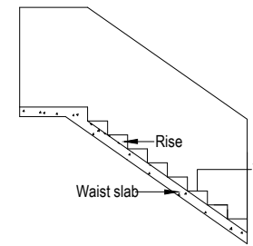
DETAILS OF STAIR CASE
