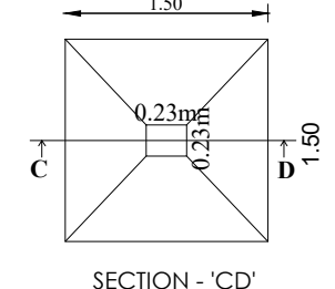
SECTION - 'CD'
