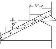
Staircase Detail Not To Scale
