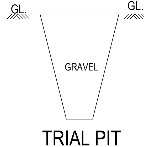
TRIAL PIT
