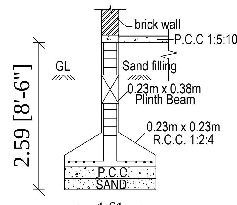
FOUNDATION DETAILS
