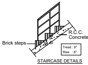
STAIRCASE DETAILS
