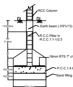
FOUNDATION DETAILS
