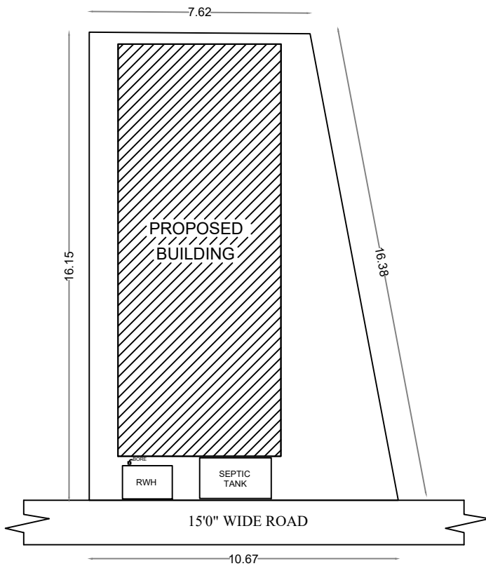
SITE PLAN
