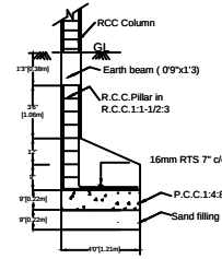
FOUNDATION DETAILS
