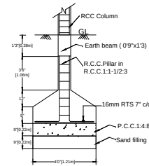
FOUNDATION DETAILS
