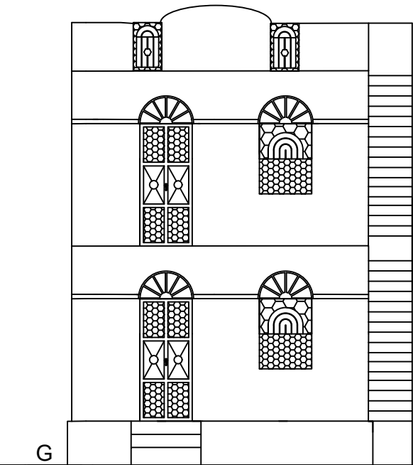
ELIVATION
