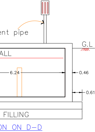
SECTION ON D-D
