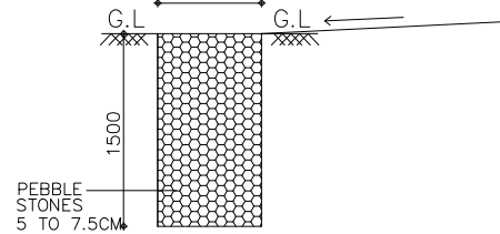
SECTION OF PEBBLE TRENCH SCALE : 1: = 100
