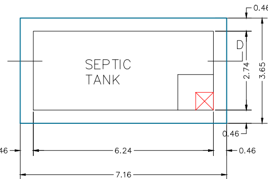
PLAN OF SEPTIC TANK SCALE 1"=2'0"
