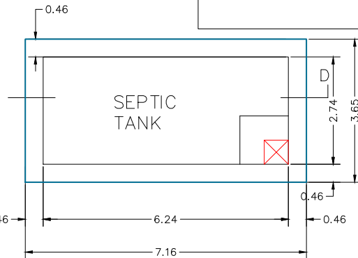
PLAN OF SEPTIC TANK SCALE 1"=2'0"
