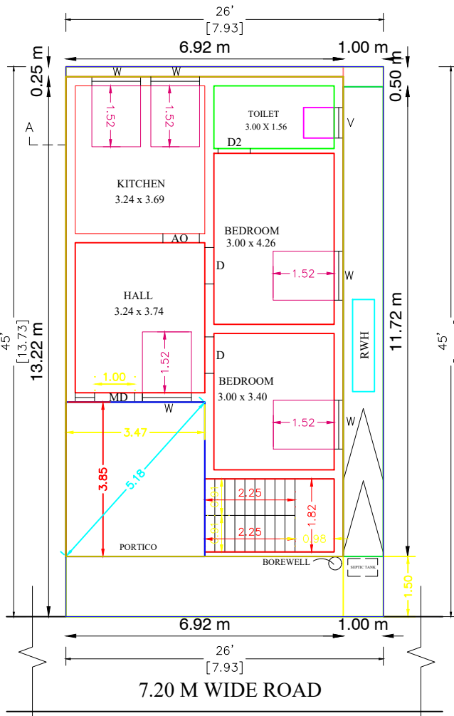
PRO.GROUND FLOOR PLAN
