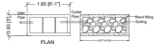
DETAILS OF SEPTIC TANK & DISPERSION TRENCH
