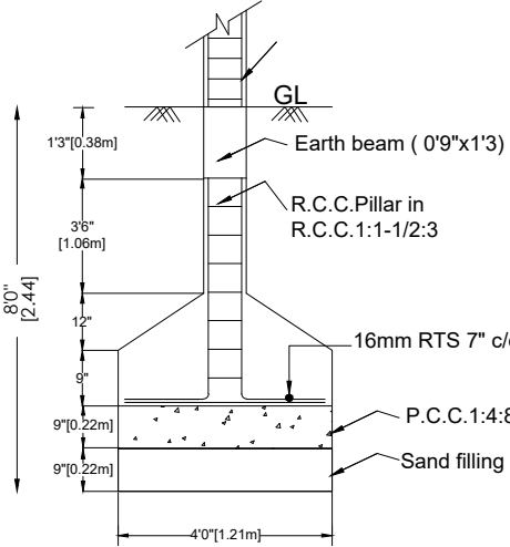
FOUNDATION DETAILS
