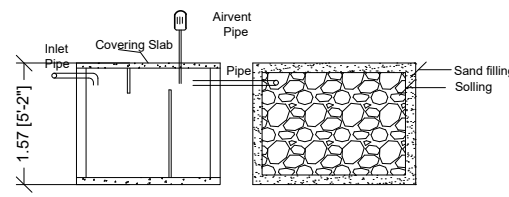
SECTION
