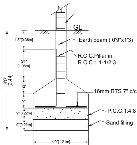
FOUNDATION DETAILS
