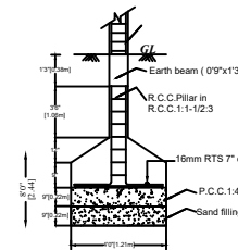
FOUNDATION DETAILS
