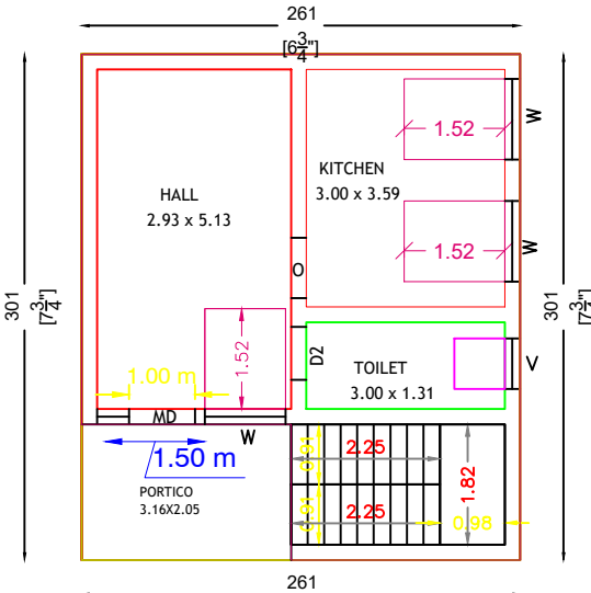
PRO.FIRST FLOOR PLAN
