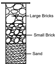
SECTION OF RAIN WATER COLLECTION PITS (NTS)
