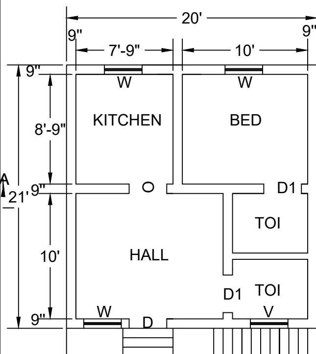
G.F. PLAN
