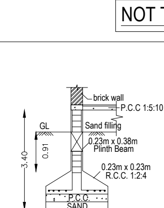
FOUNDATION DETAILS
