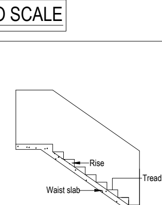
DETAILS OF STAIR CASE
