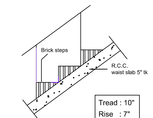
STAIRCASE DETAILS-NTS
