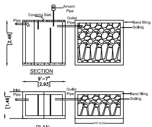
TRIAL PIT.
