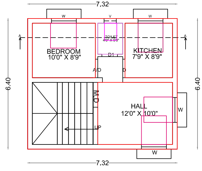
PRO.,SECOND FLOOR PLAN (RESIDENTIAL)
