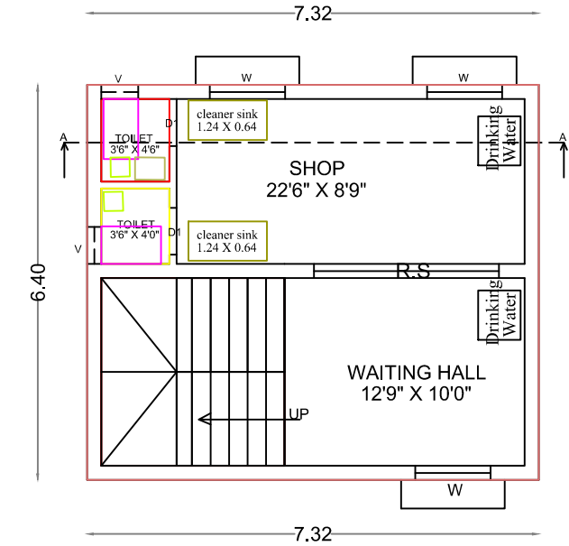
PRO.,FIRST FLOOR PLAN (COMMERICAL)
