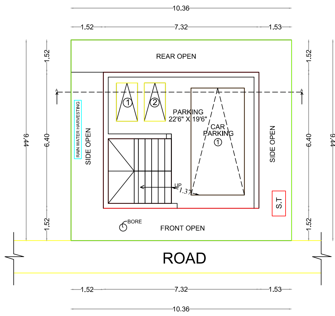
SITE / PRO.,STILT FLOOR PLAN (COMMERICAL)
