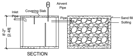
DETAILS OF SEPTIC TANK & DISPERSION TRENCH
