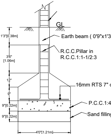
FOUNDATION DETAILS
