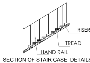
SECTION OF STAIR CASE DETAILS
