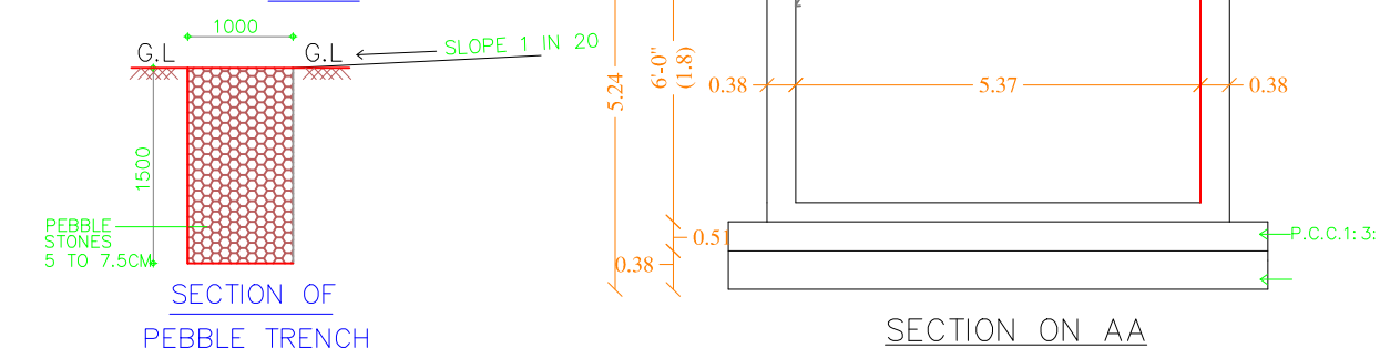
COMPOUND WALL DETAIL
