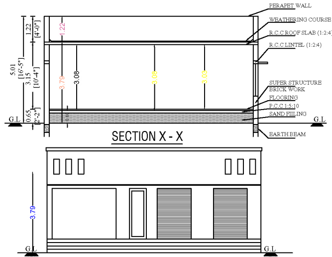
ELEVATION 50'0" (15.24)
