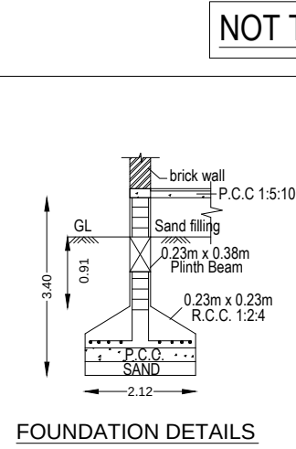
FOUNDATION DETAILS
