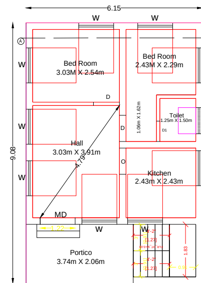
PROPOSED GROUND FLOOR
