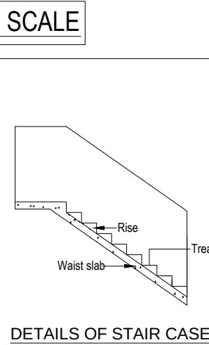
DETAILS OF STAIR CASE
