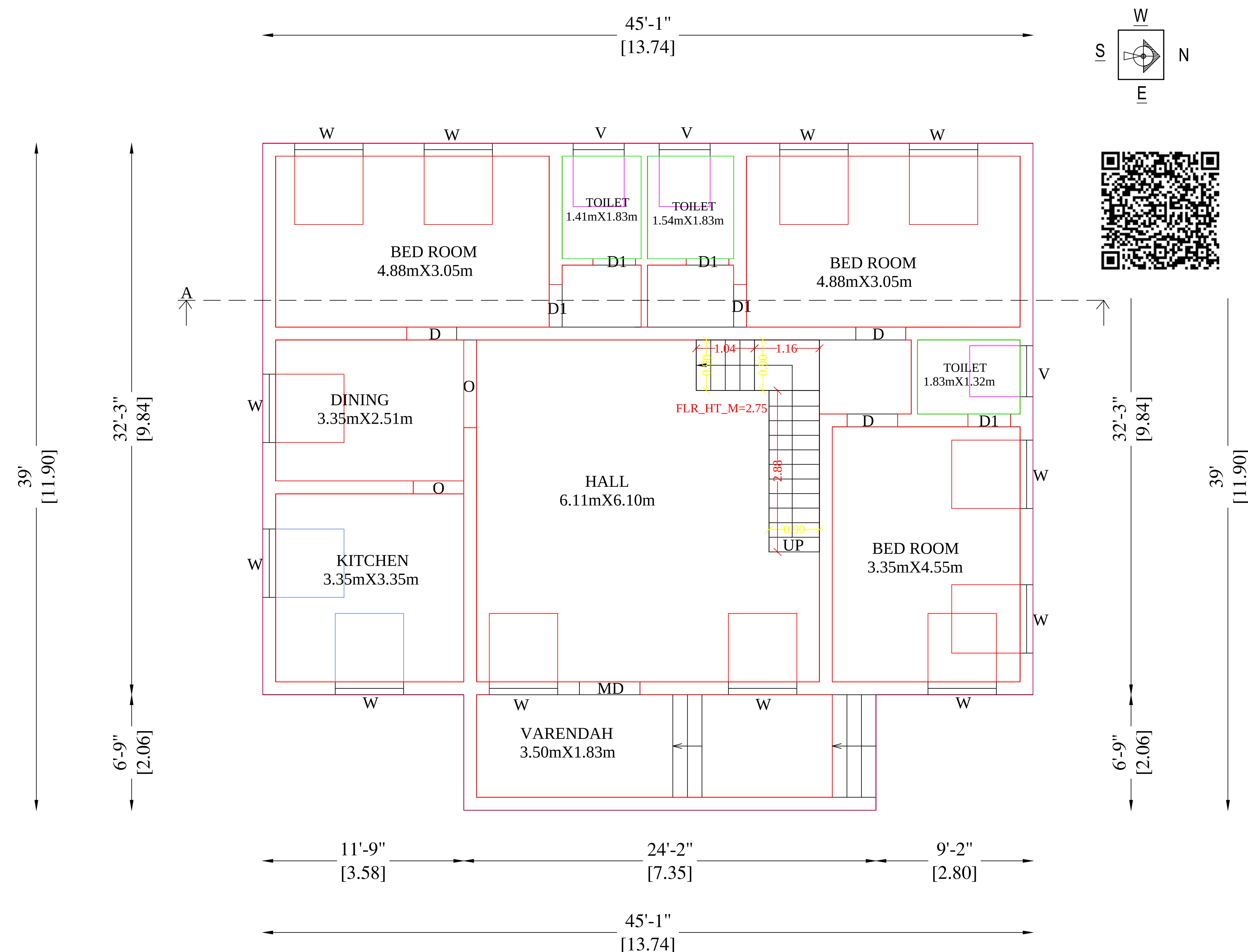
PRO. GROUND FLOOR PLAN
