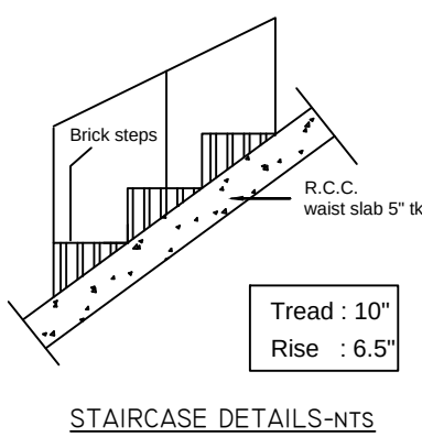
STAIRCASE DETAILS-NTS
