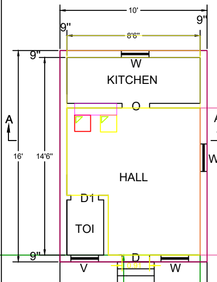
G.F. PLAN
