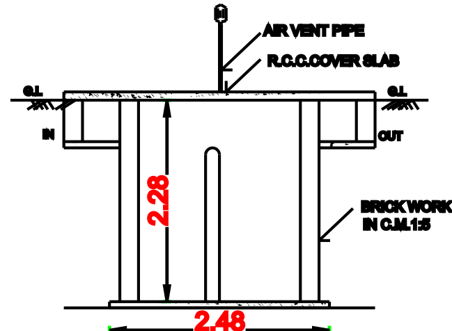
SEPTIC TANK DETAILS-SECTION
