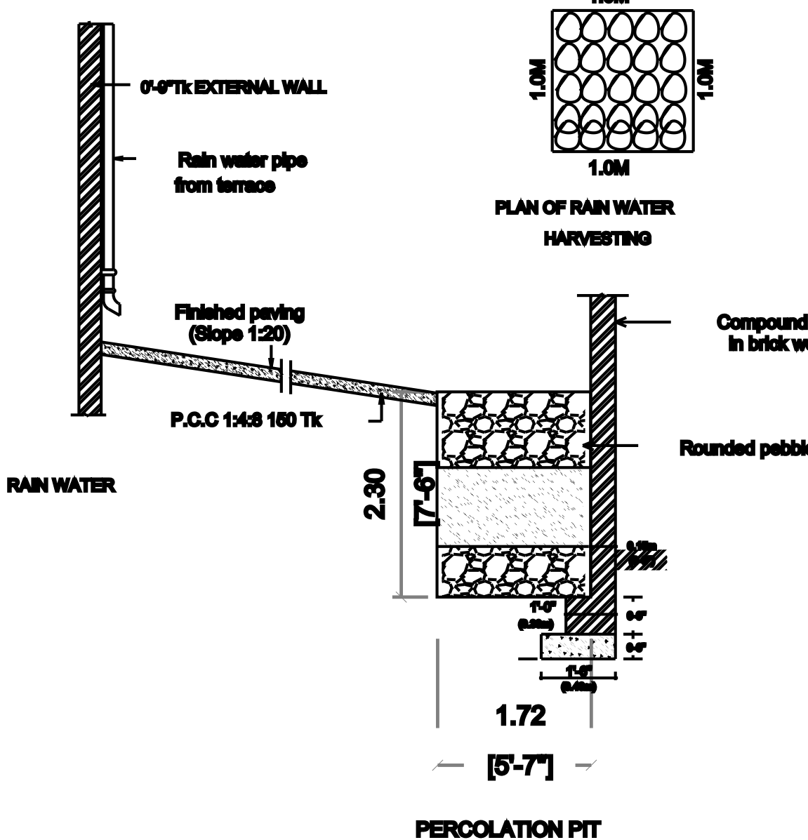
PERCOLATION PIT
