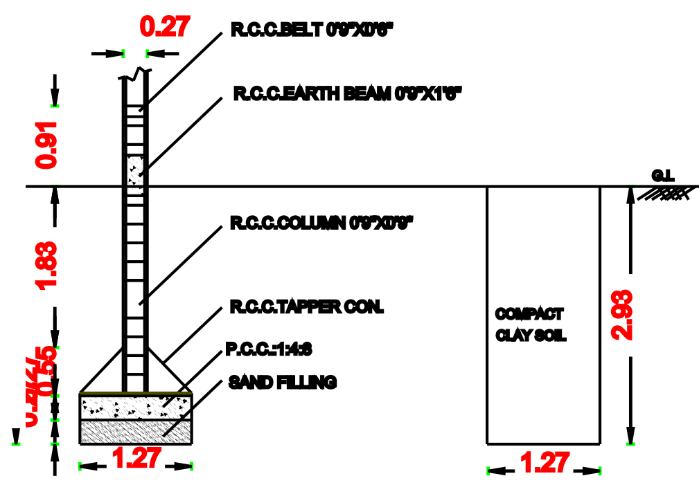
FOUNDATION DETAILS-MIDDLE COLUMN
