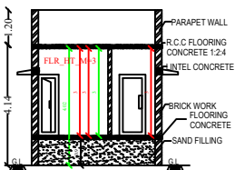
SECTION ON 'AA'
