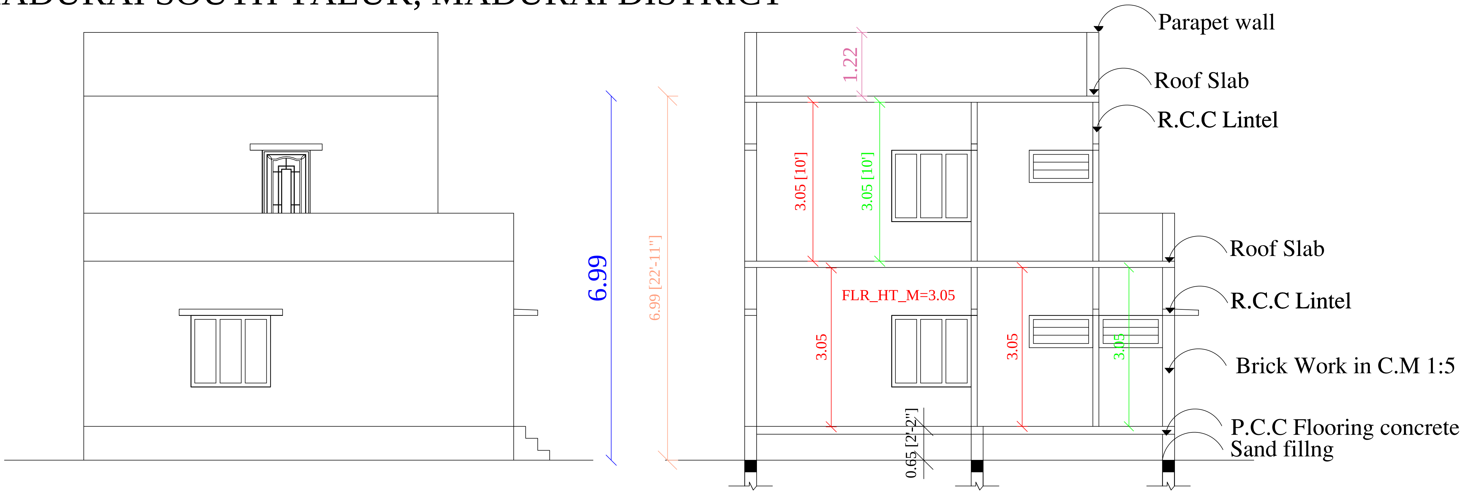
FRONT ELEVATION
