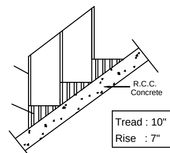
STAIRCASE DETAILS
