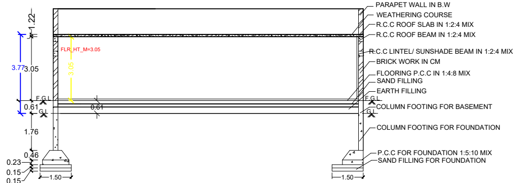
SECTION ON-AA
