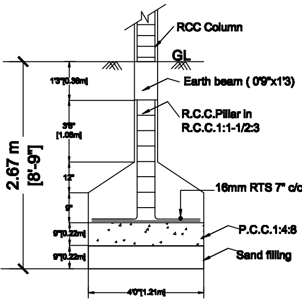
FOUNDATION DETAILS
