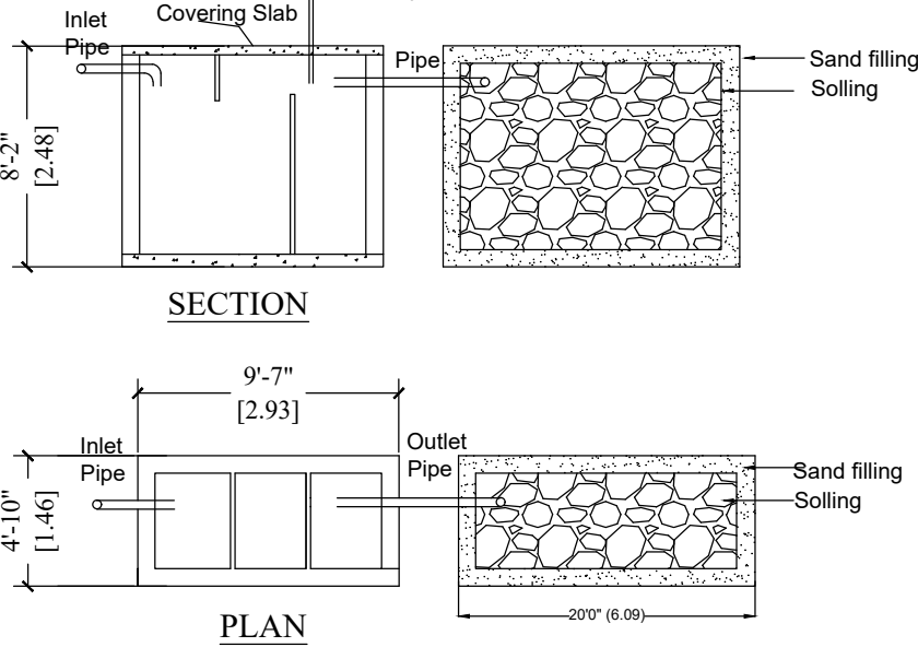
DETAILS OF SEPTIC TANK & DISPERSION TRENCH
