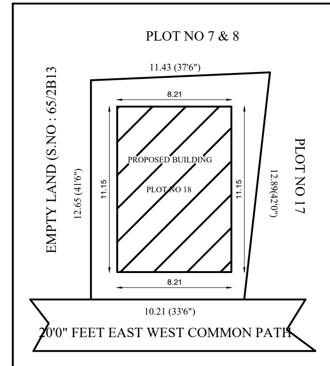
SITE PLAN
