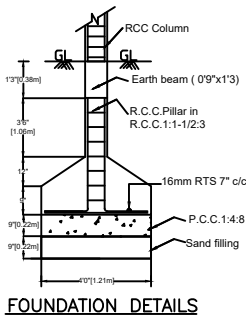
FOUNDATION DETAILS
