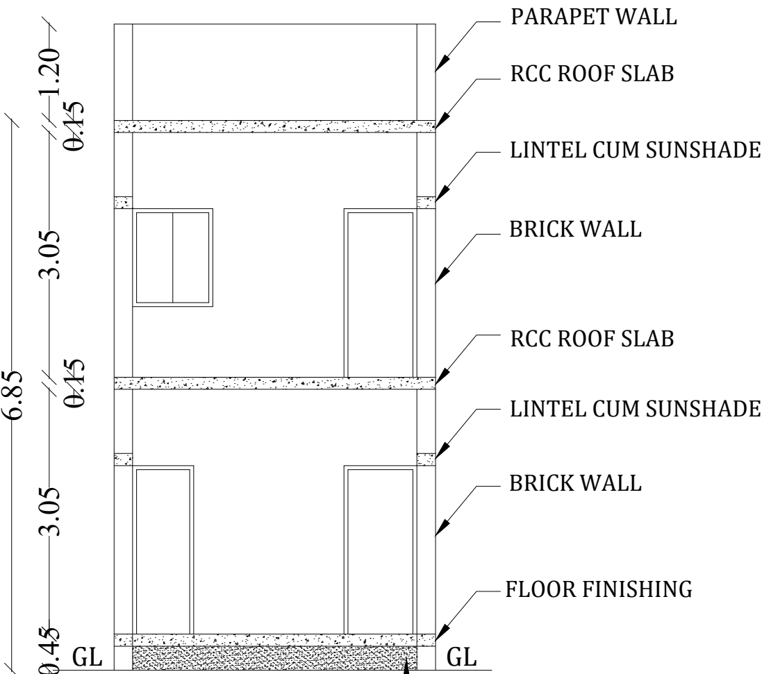
SECTION -AA
