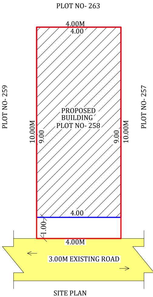
SITE PLAN
