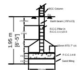
FOUNDATION DETAILS
