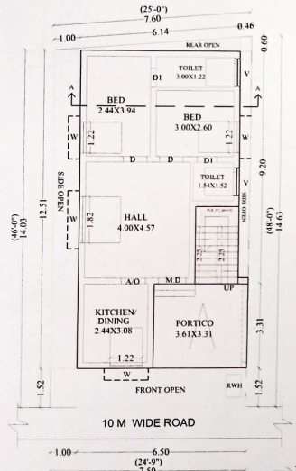
PRO-GROUND FLOOR PLAN
