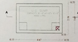
SUMP DETAIL
