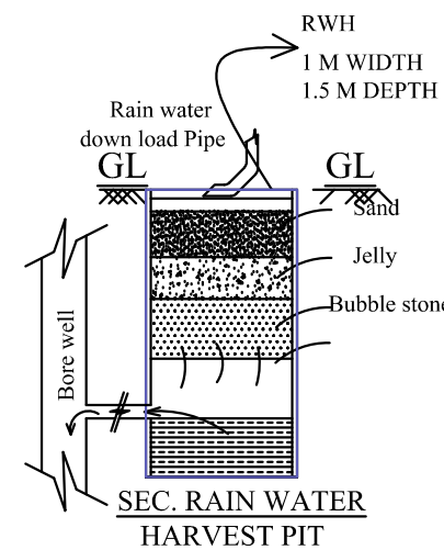
SEC. RAIN WATER HARVEST PIT
