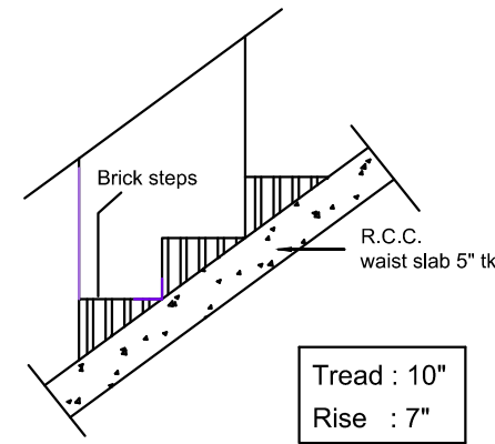
STAIRCASE DETAILS-NTS
