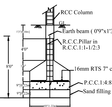
FOUNDATION DETAILS
