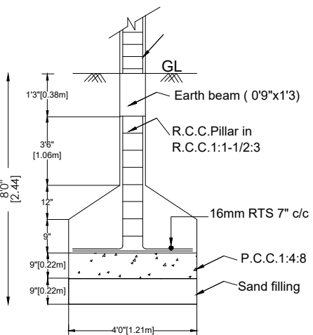
FOUNDATION DETAILS
