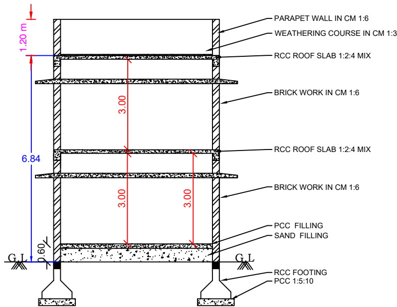
SECTION AB
