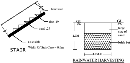
RAINWATER HARVESTING
