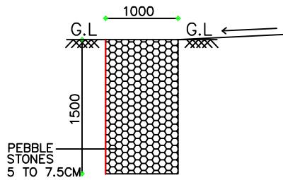
SECTION OF PEBBLE TRENCH SCALE : 1: = 100
