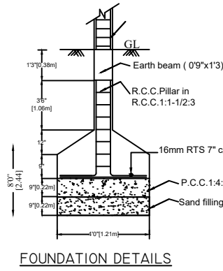
FOUNDATION DETAILS
