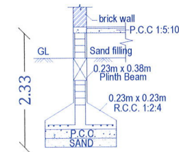
FOUNDATION DETAILS
