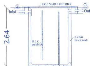
SECTION OF SEPTIC TANK
