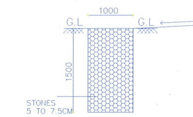
SECTION OF PEBBLE TRENCH
