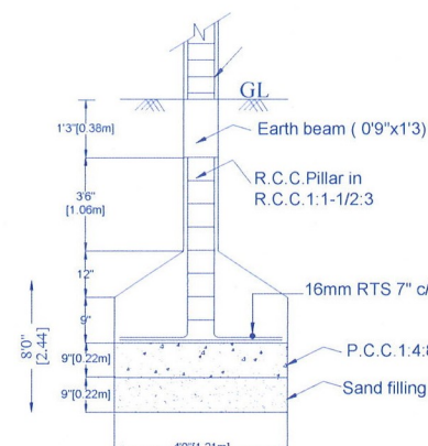
FOUNDATION DETAILS
